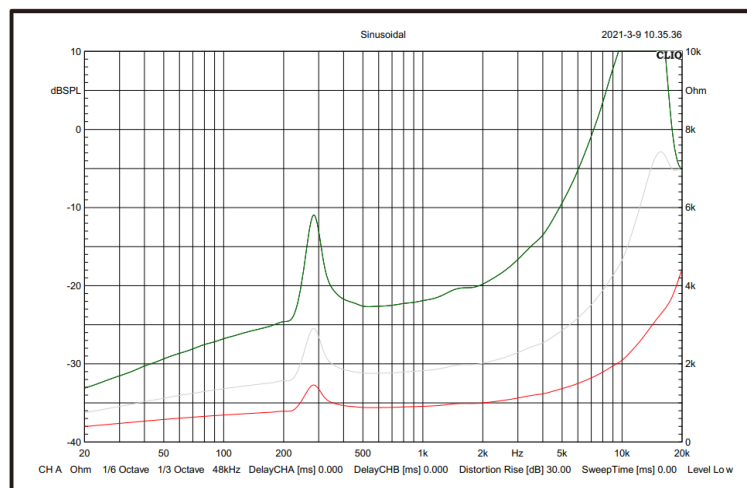
[ Impedance diagram ]
