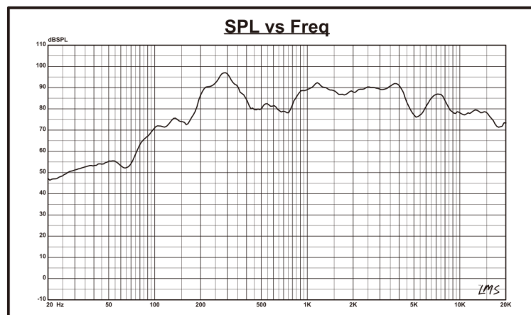
[ Frequency response diagram ]
